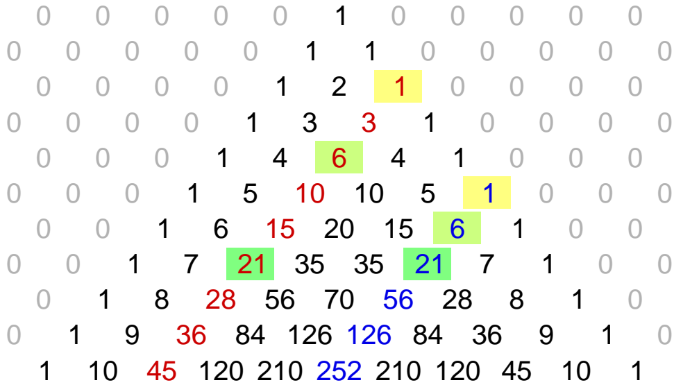
FIGURE 1. Pascal's Triangle
