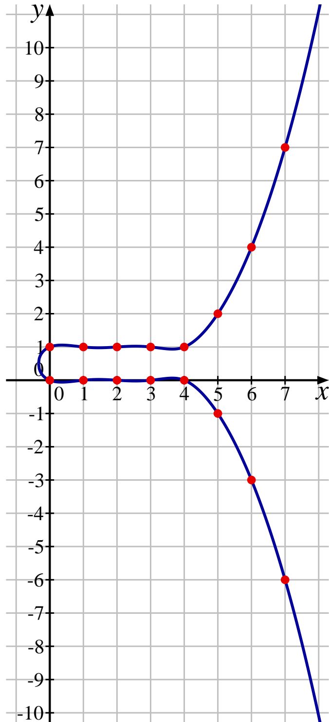
FIGURE 2. The curve given by (2.2), with some integral points.
